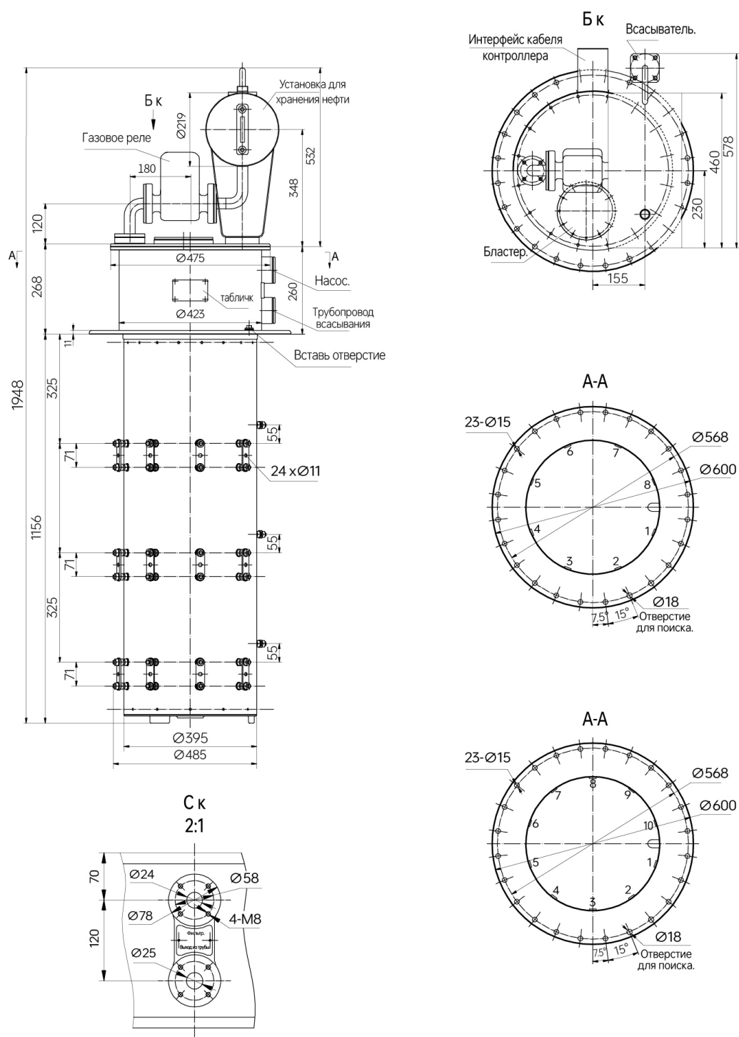
SY1-D400/35-7x7 SY1-D400/35-9x9
