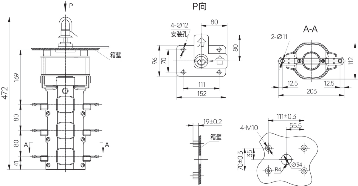
图1 ARF1-10/630 (315)-20-II
