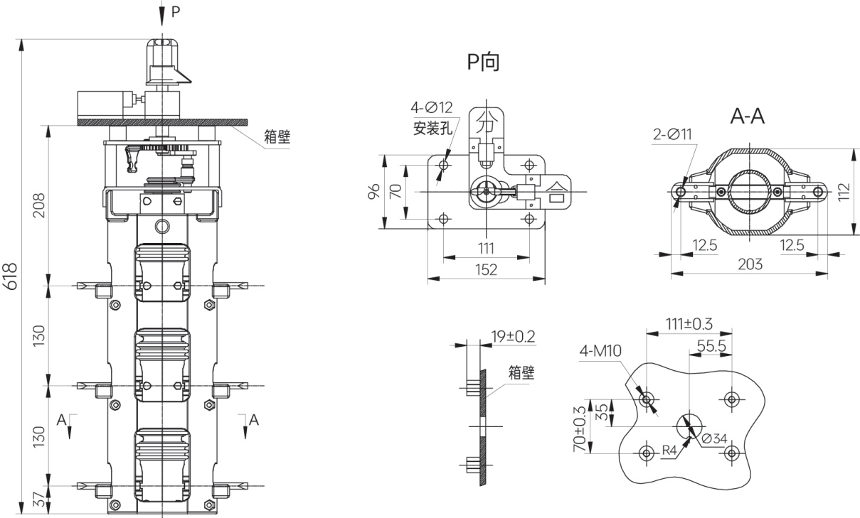
图2 ARF1-35/630 (315)-20-II
